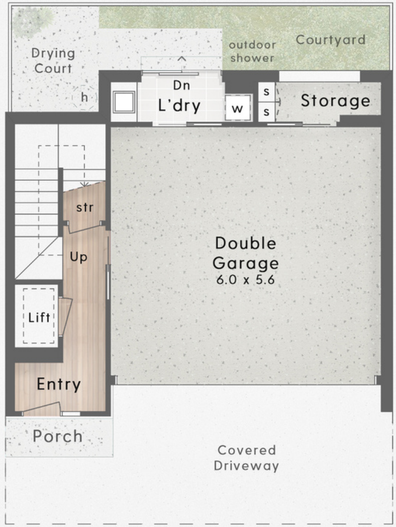
:: FLOOR PLAN Ground Floor - 2.6m Ceiling
