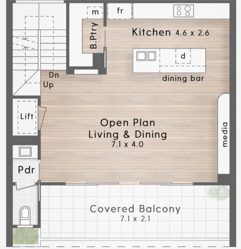
:: FLOOR PLAN Second Floor - 2.7m Ceiling
