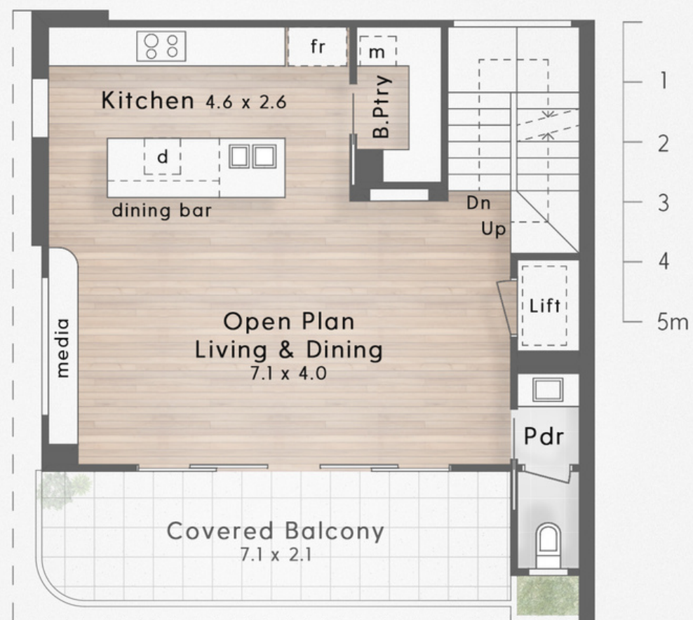
:: FLOOR PLAN Second Floor - 2.7m Ceiling
