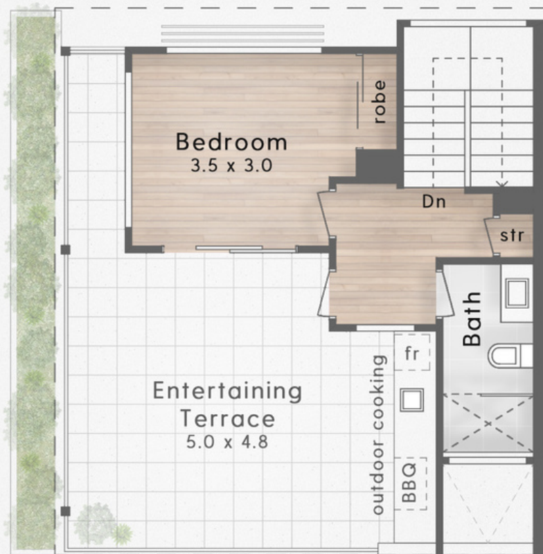
:: FLOOR PLAN Third Floor - 2.6m Ceiling
