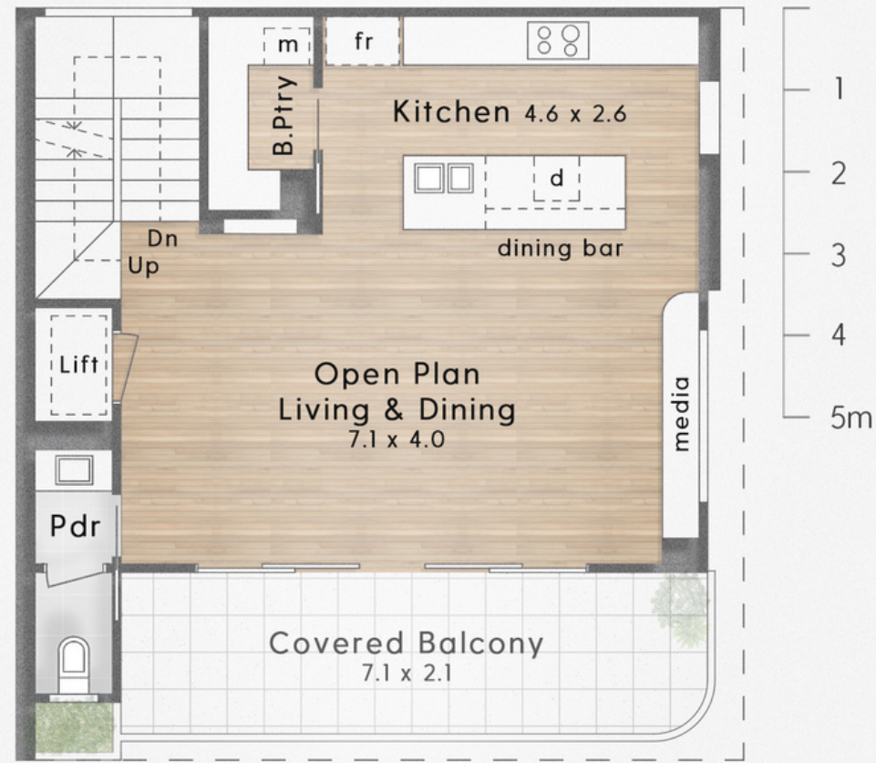
:: FLOOR PLAN Second Floor
